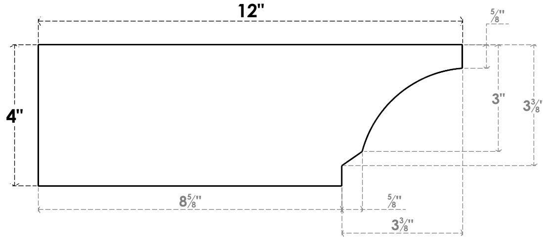
SIDE PROFILE
